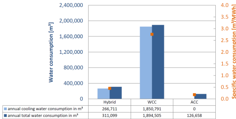
Simulation-based water demand comparison of different cooling technologies of a 100MW CRS plant.
