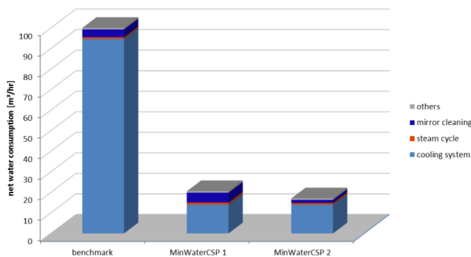
Comparison of the identified benchmark with the suggested MinWaterCSP water management concepts with and without re-use cycles.
